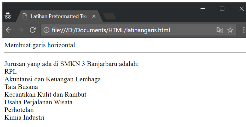
Gambar 1.9 Tampilan program 1.9
