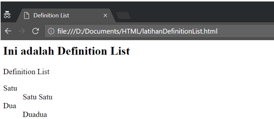
Gambar 1.11 Tampilan program 1.12
