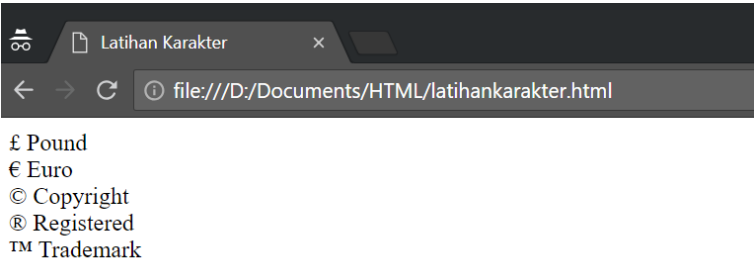
Gambar 1.7 Tampilan program 1.7
