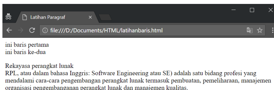
Gambar 1.5 Tampilan program 1.5
