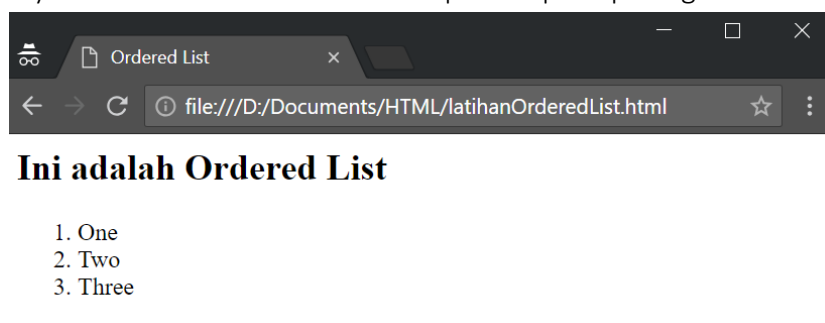
Gambar 1.10 Tampilan program 1.10
