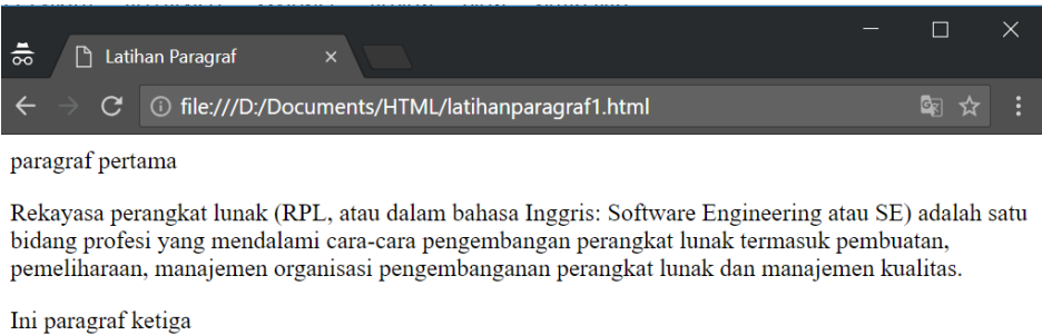
Gambar 1.3 Tampilan program 1.3
