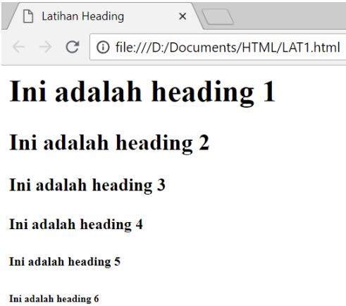
Gambar 1.1 Tampilan program 1.1
