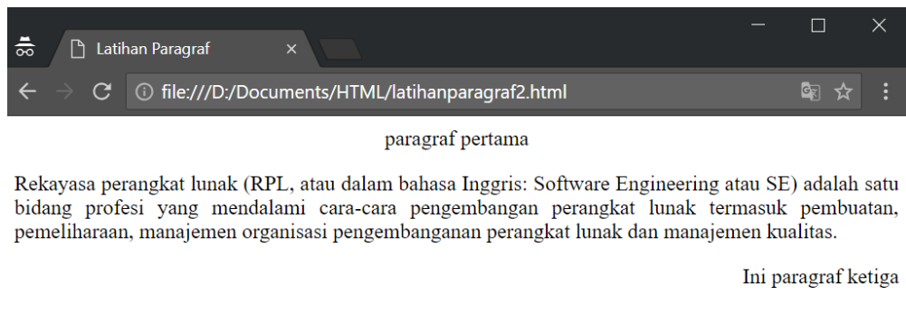
Gambar 1.4 Tampilan program 1.4
