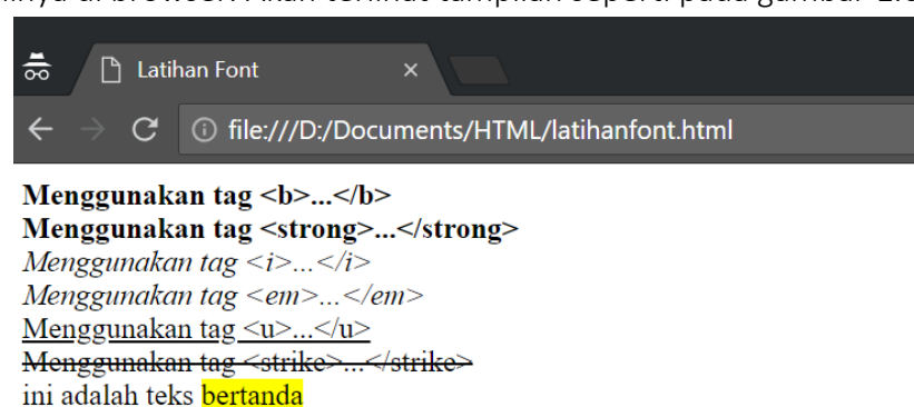
Gambar 1.6 Tampilan program 1.6
